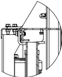
DETAIL D SCALE 1 : 9
